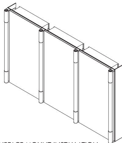
SURFACE MOUNT INSTALLATION 51-3/4" x 30"
