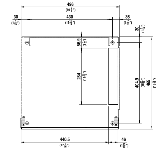
TOP VIEW (FRONT COVER REMOVED FOR CLARITY)
