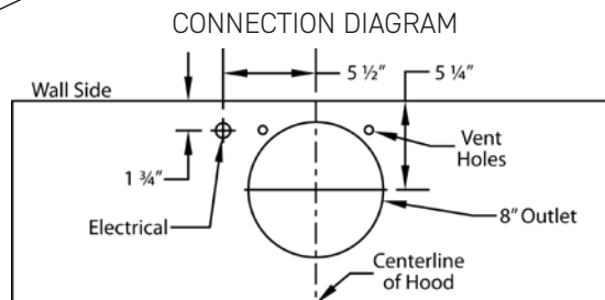
600 CFM B200 Dual Blower (Top View)
